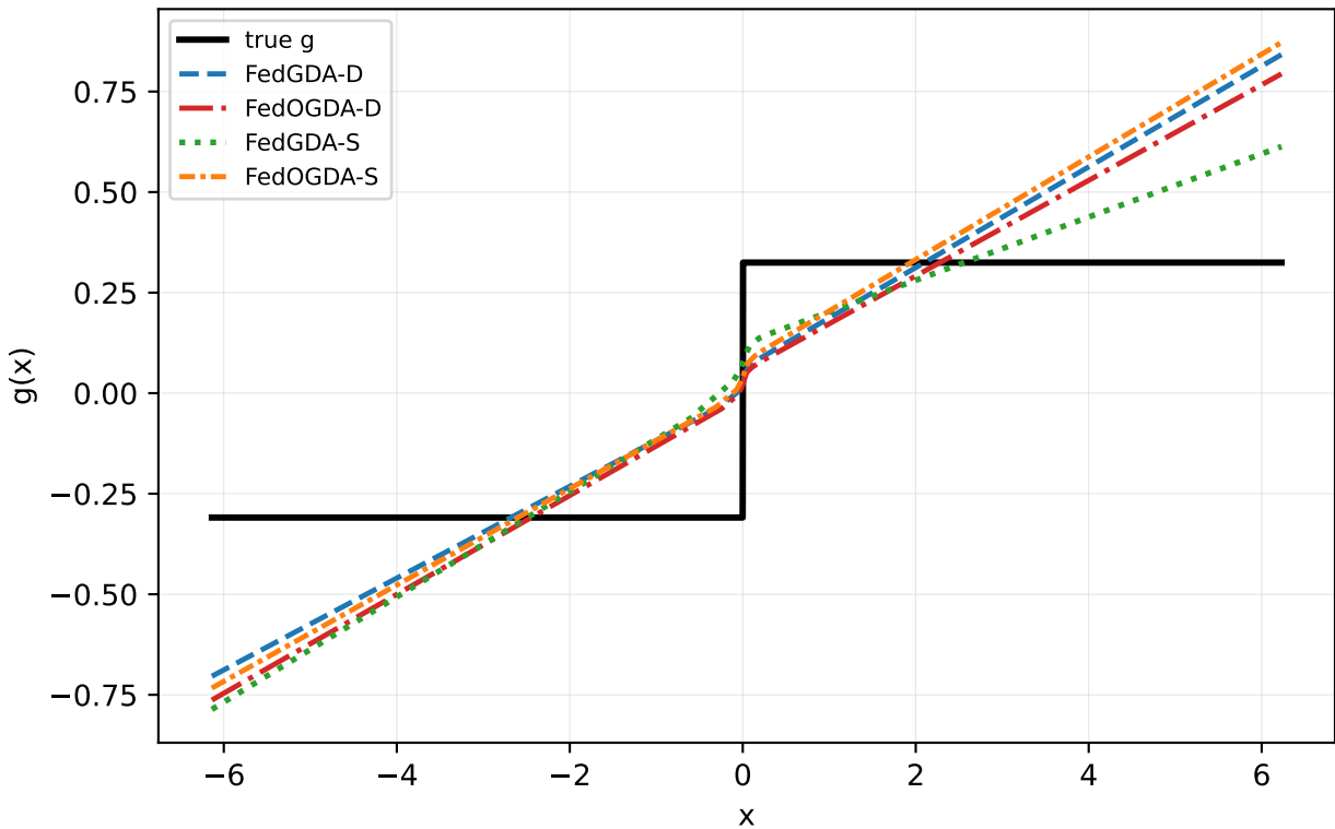
Step alpha=0.5 seed=1: all federated methods
