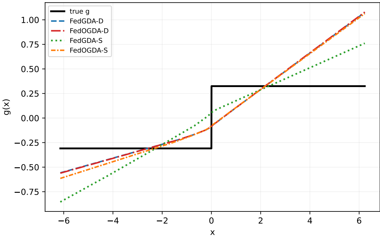
Step alpha=1.0 seed=2: all federated methods
