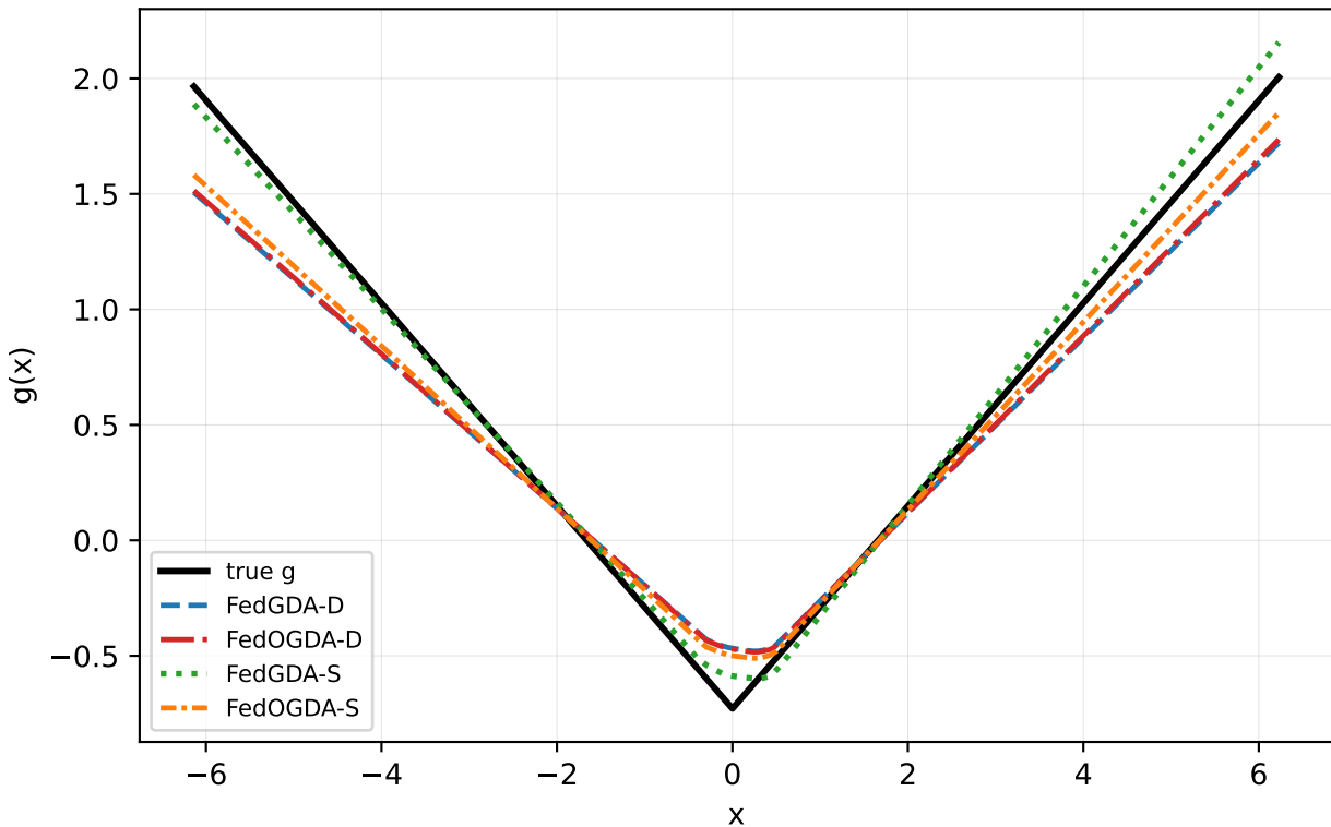
Absolute alpha=0.1: mean all federated methods
