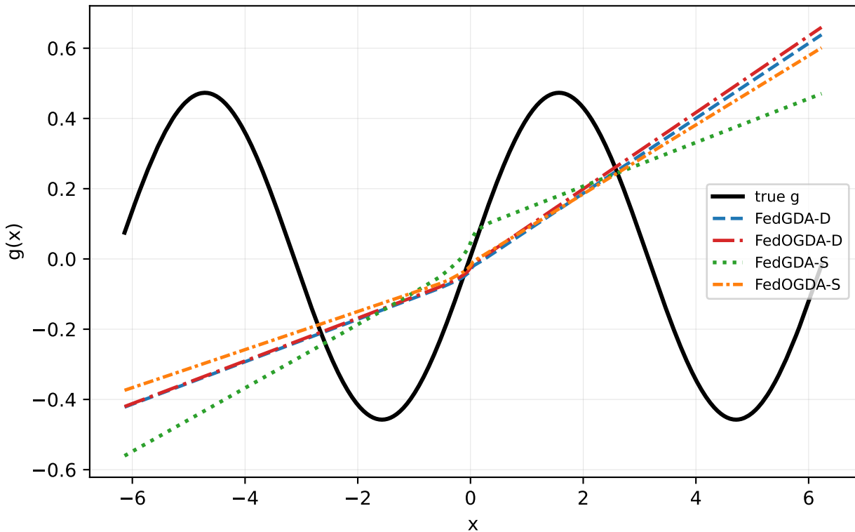
Sine \alpha=0.1 : mean all federated methods
