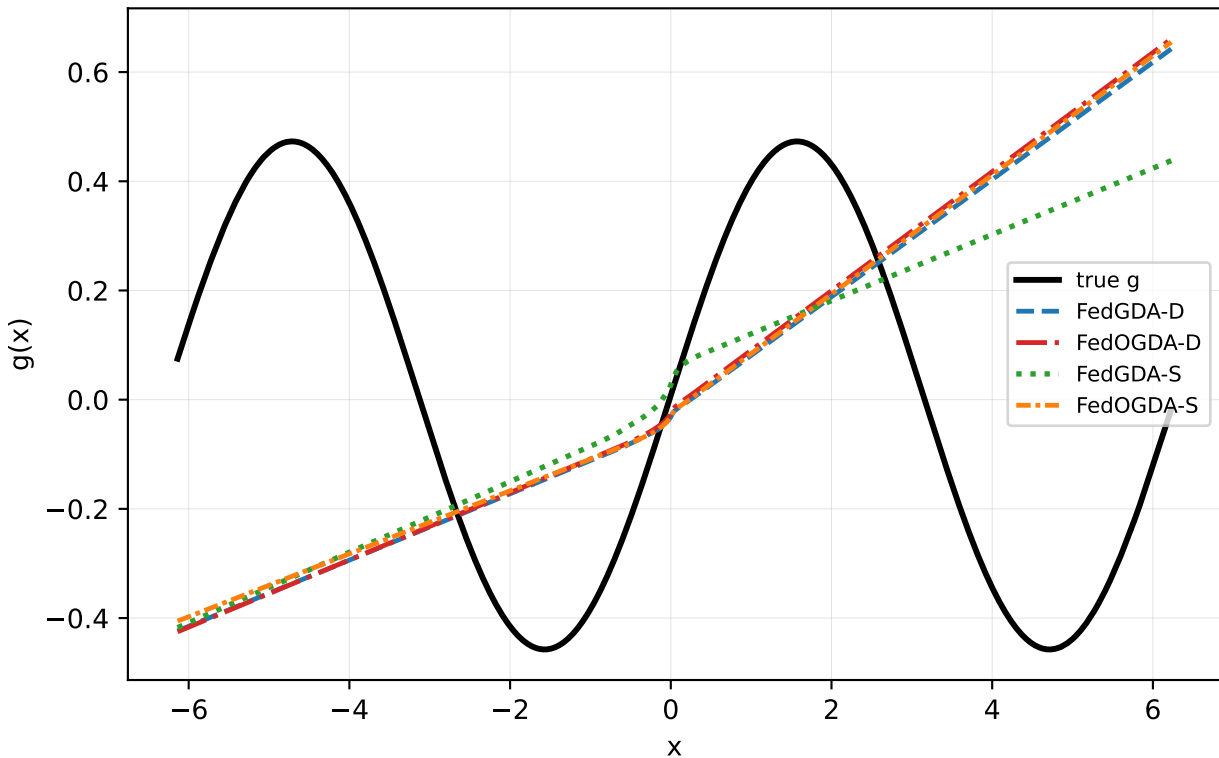
Sine \alpha=0.5 : mean all federated methods
