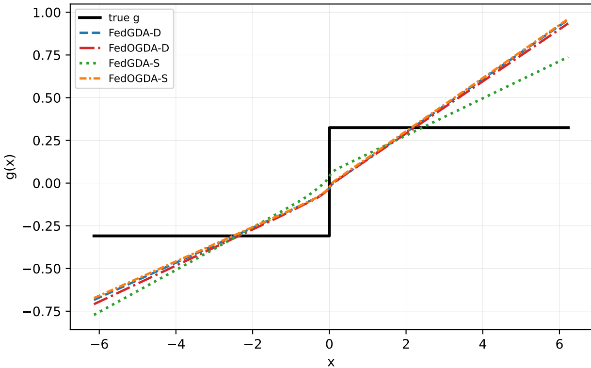
Step alpha=0.5: mean all federated methods
