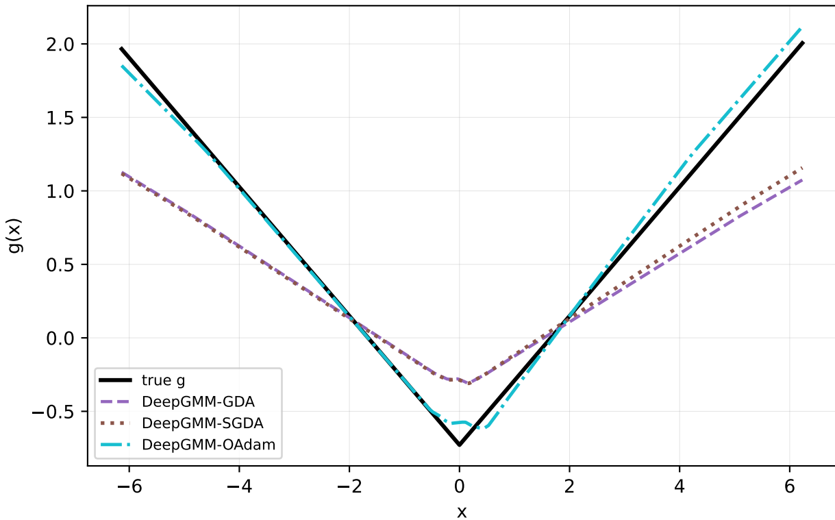
Absolute centralized seed=0: GDA vs SGDA vs OAdam
