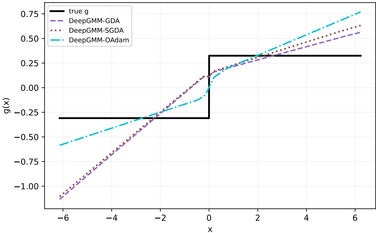
Step centralized seed=0: GDA vs SGDA vs OAdam
