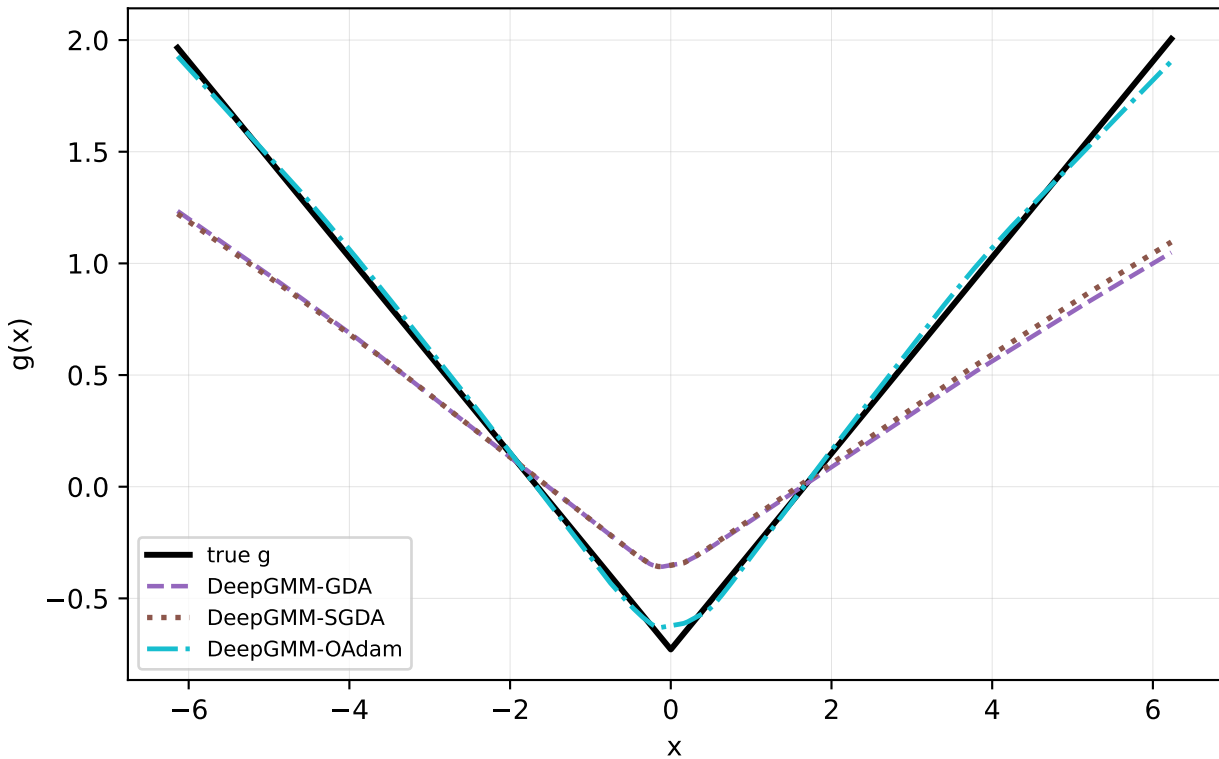
Absolute centralized: mean GDA/SGDA/OAdam
