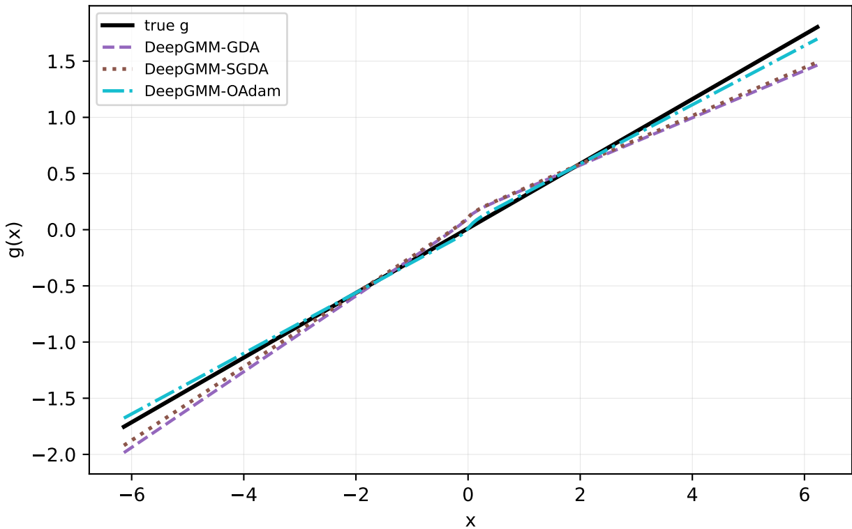
Linear centralized: mean GDA/SGDA/OAdam
