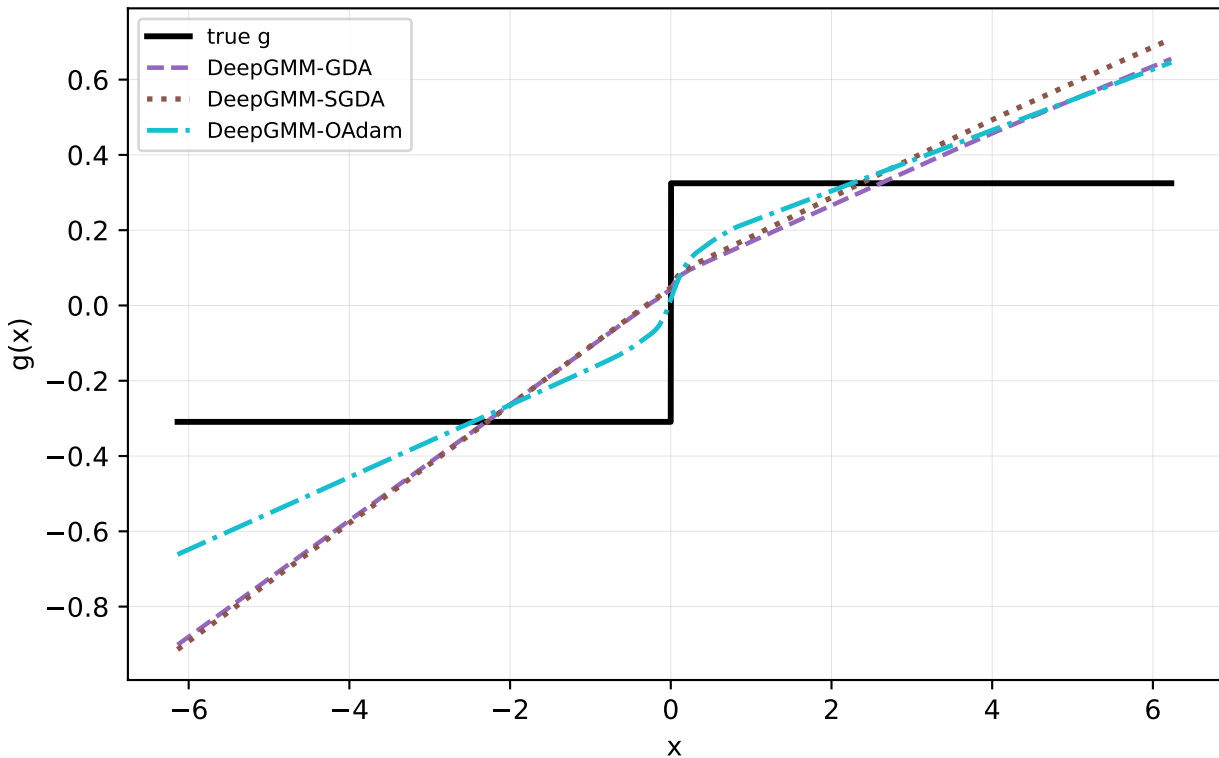
Step centralized: mean GDA/SGDA/OAdam
