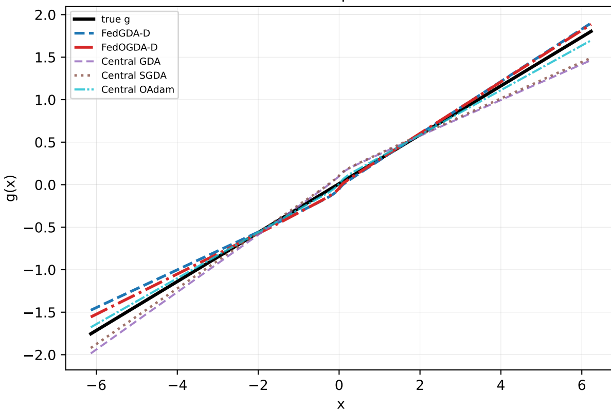
Linear alpha=0.1
