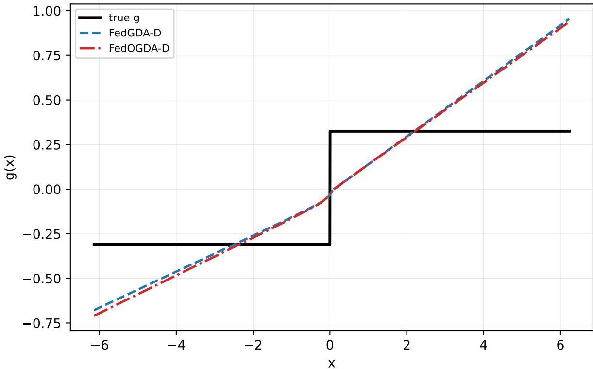
Step summary curve (base_sweep, alpha=0.1)
