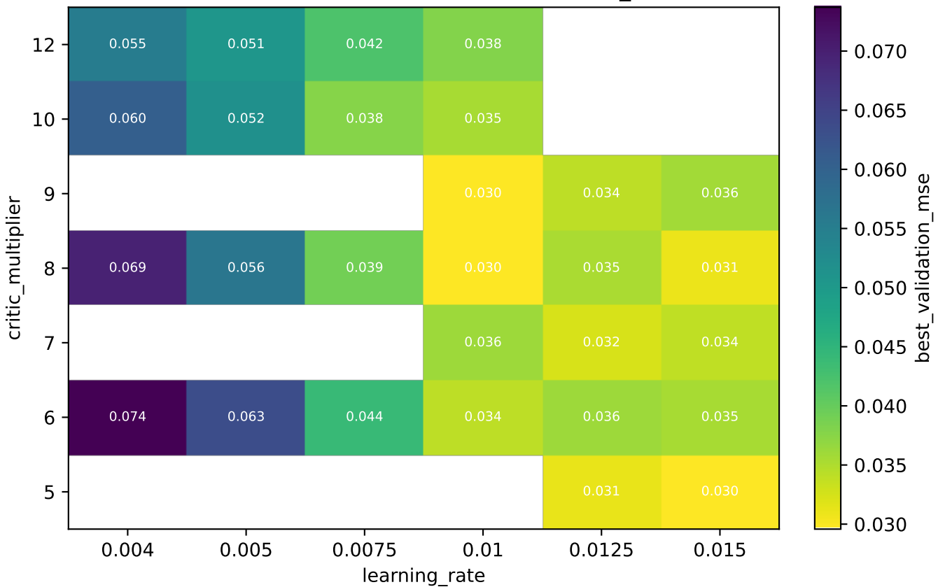
Sine validation MSE, lambda=0.01, server_lr=1.5
