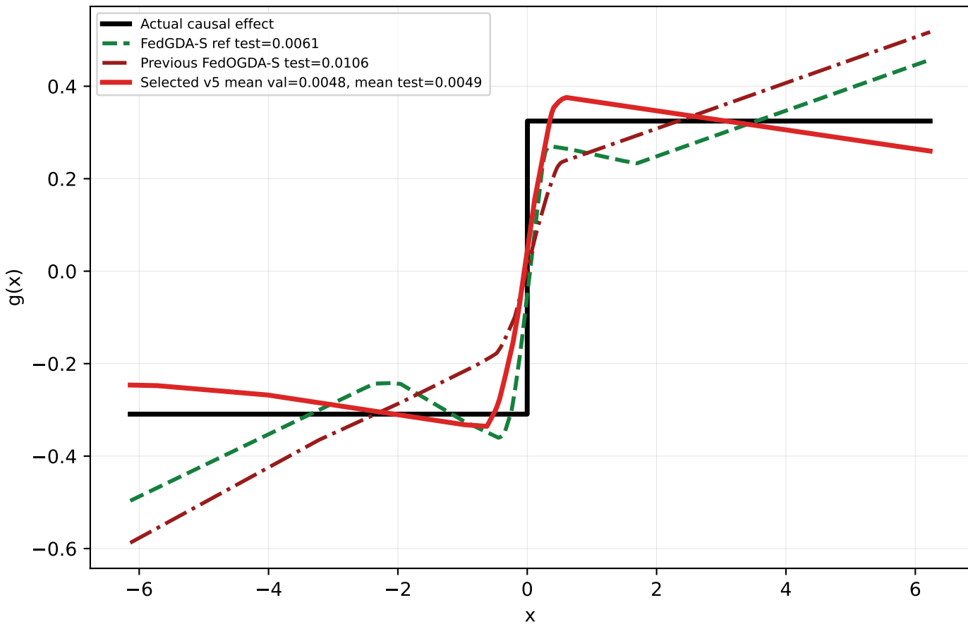
Step \alpha=0.5 : validation-selected FedOGDA-S v5 \text{lr}=0.0075 , \text{cm}=20 , \text{lambda}=0.05 , \text{server\_lr}=1 , T=1500 , R=7
