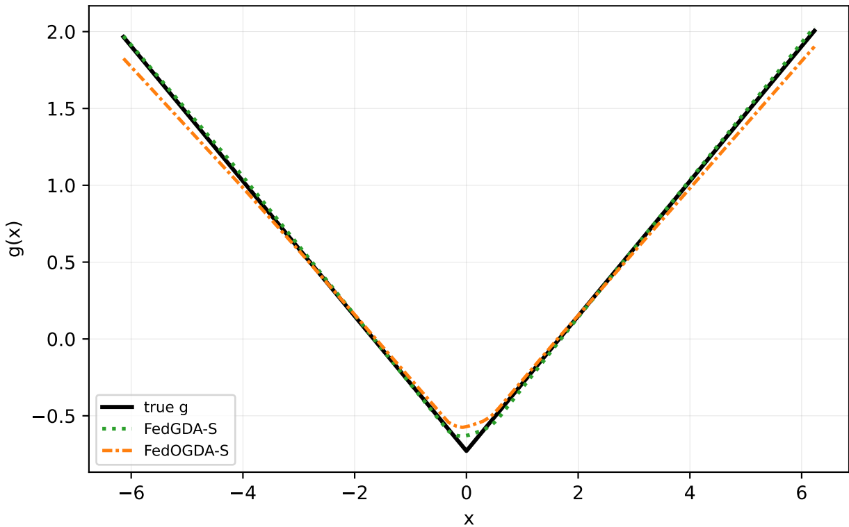
Absolute alpha=0.5 seed=0: FedGDA-S vs tuned FedOGDA-S
