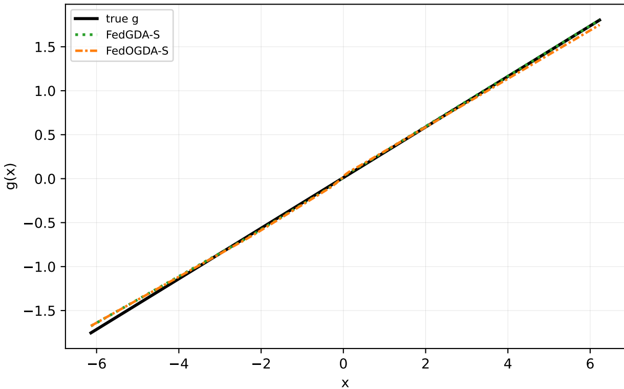
Linear alpha=0.5 seed=0: FedGDA-S vs tuned FedOGDA-S
