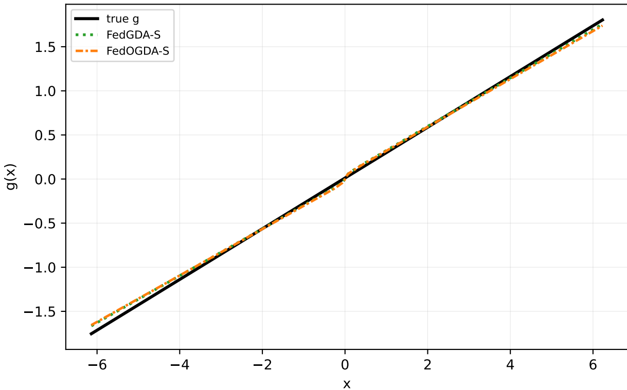
Linear alpha=0.5 seed=1: FedGDA-S vs tuned FedOGDA-S
