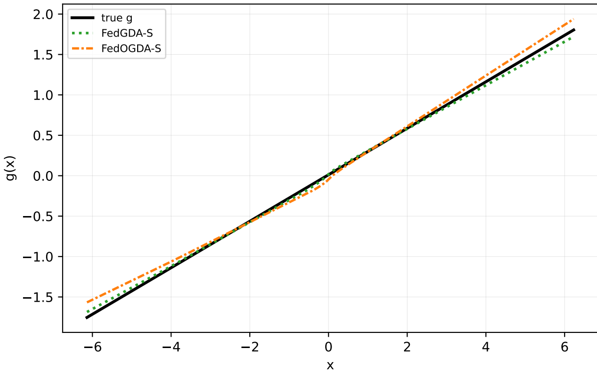
Linear alpha=0.5 seed=2: FedGDA-S vs tuned FedOGDA-S
