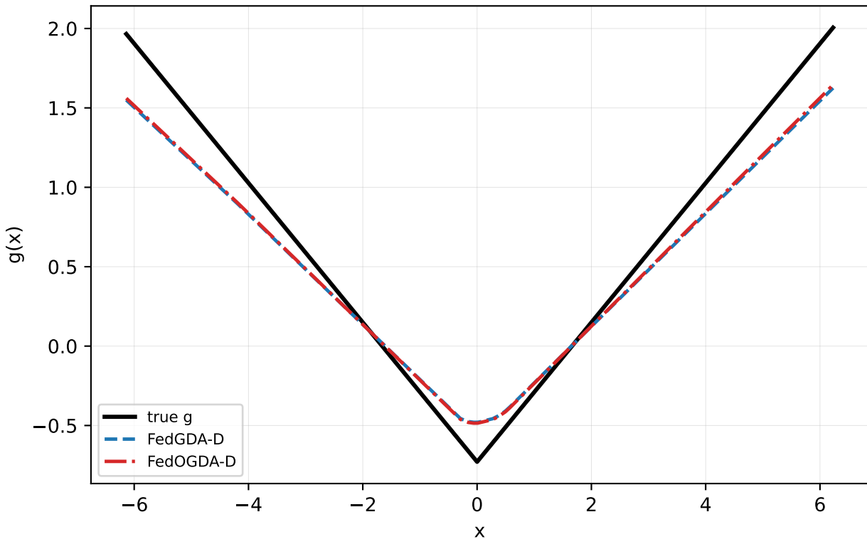
Absolute alpha=0.1 seed=0: FedGDA-D vs FedOGDA-D
