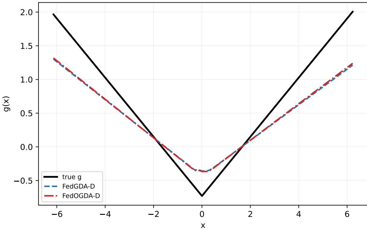
Absolute alpha=0.1 seed=2: FedGDA-D vs FedOGDA-D
