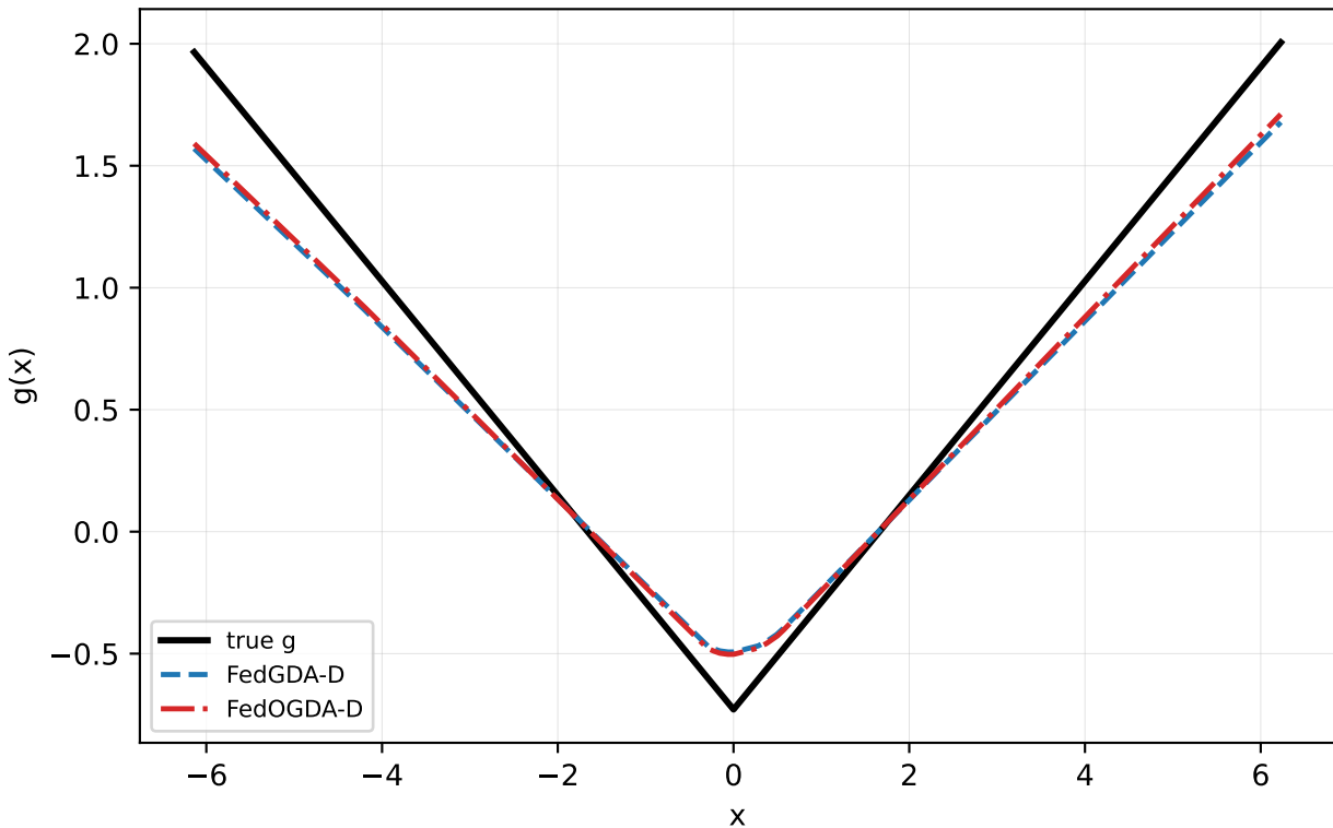
Absolute alpha=1.0 seed=0: FedGDA-D vs FedOGDA-D
