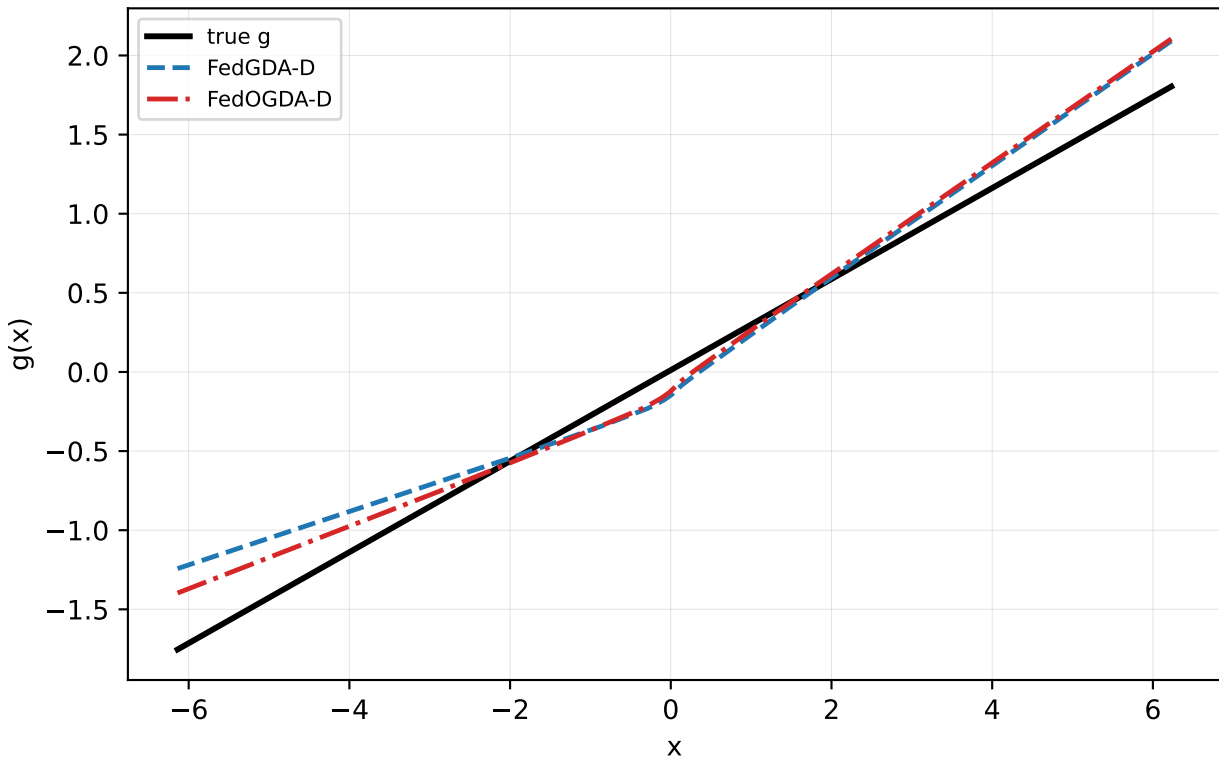
Linear alpha=0.1 seed=2: FedGDA-D vs FedOGDA-D
