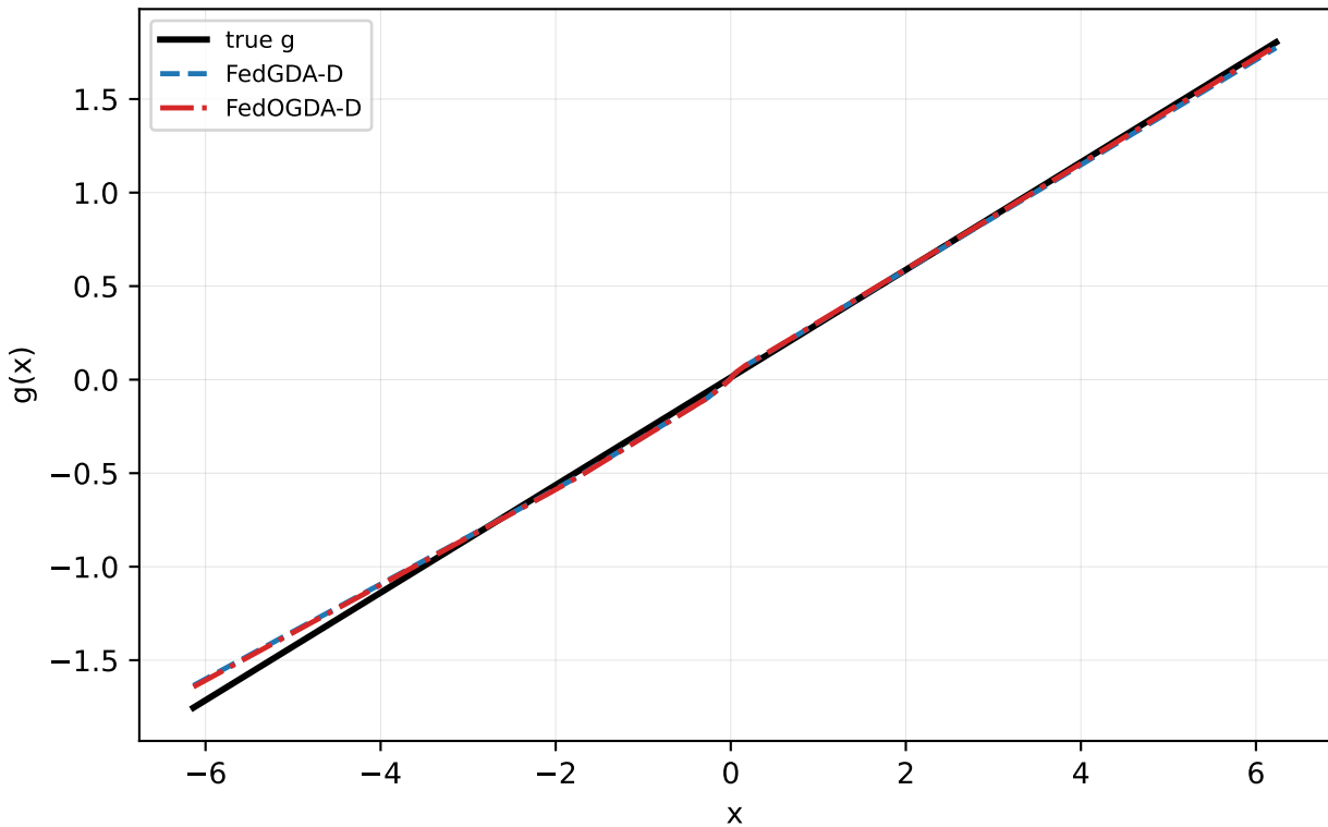
Linear alpha=0.5 seed=0: FedGDA-D vs FedOGDA-D
