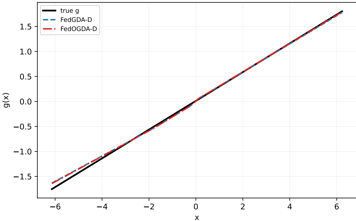
Linear alpha=1.0 seed=0: FedGDA-D vs FedOGDA-D
