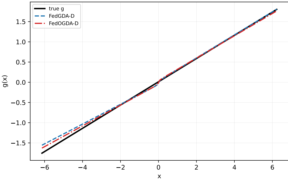
Linear alpha=1.0 seed=1: FedGDA-D vs FedOGDA-D
