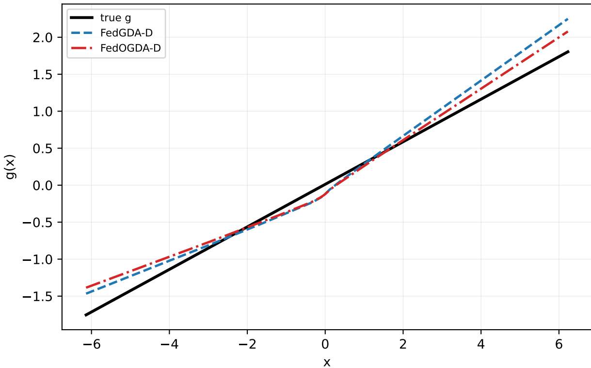
Linear alpha=1.0 seed=2: FedGDA-D vs FedOGDA-D
