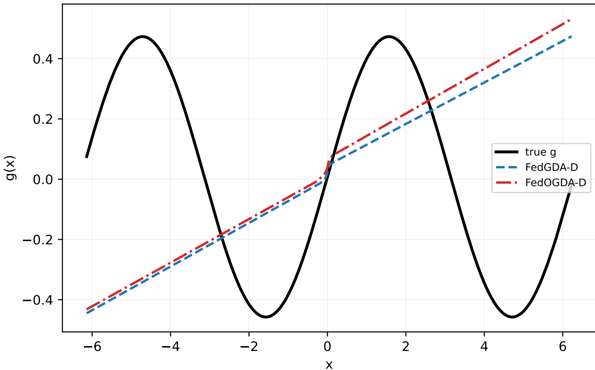
Sine \alpha=0.1 seed=1: FedGDA-D vs FedOGDA-D
