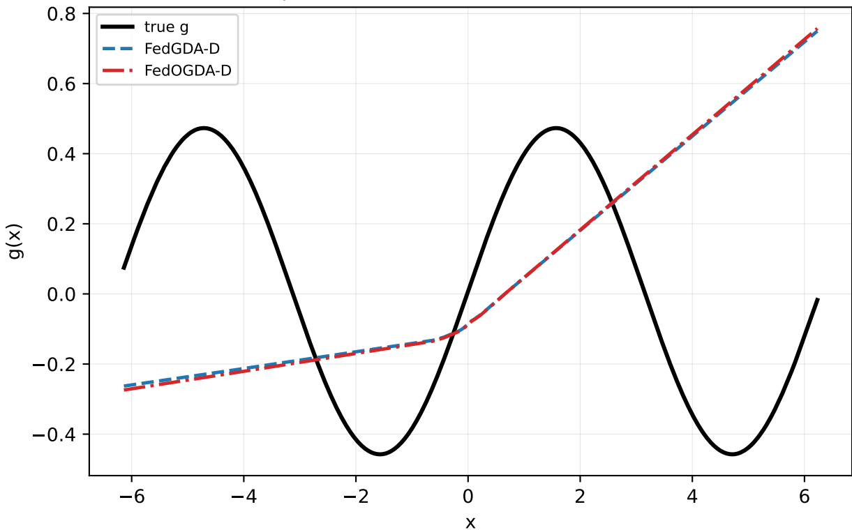
Sine \alpha=0.1 seed=2: FedGDA-D vs FedOGDA-D
