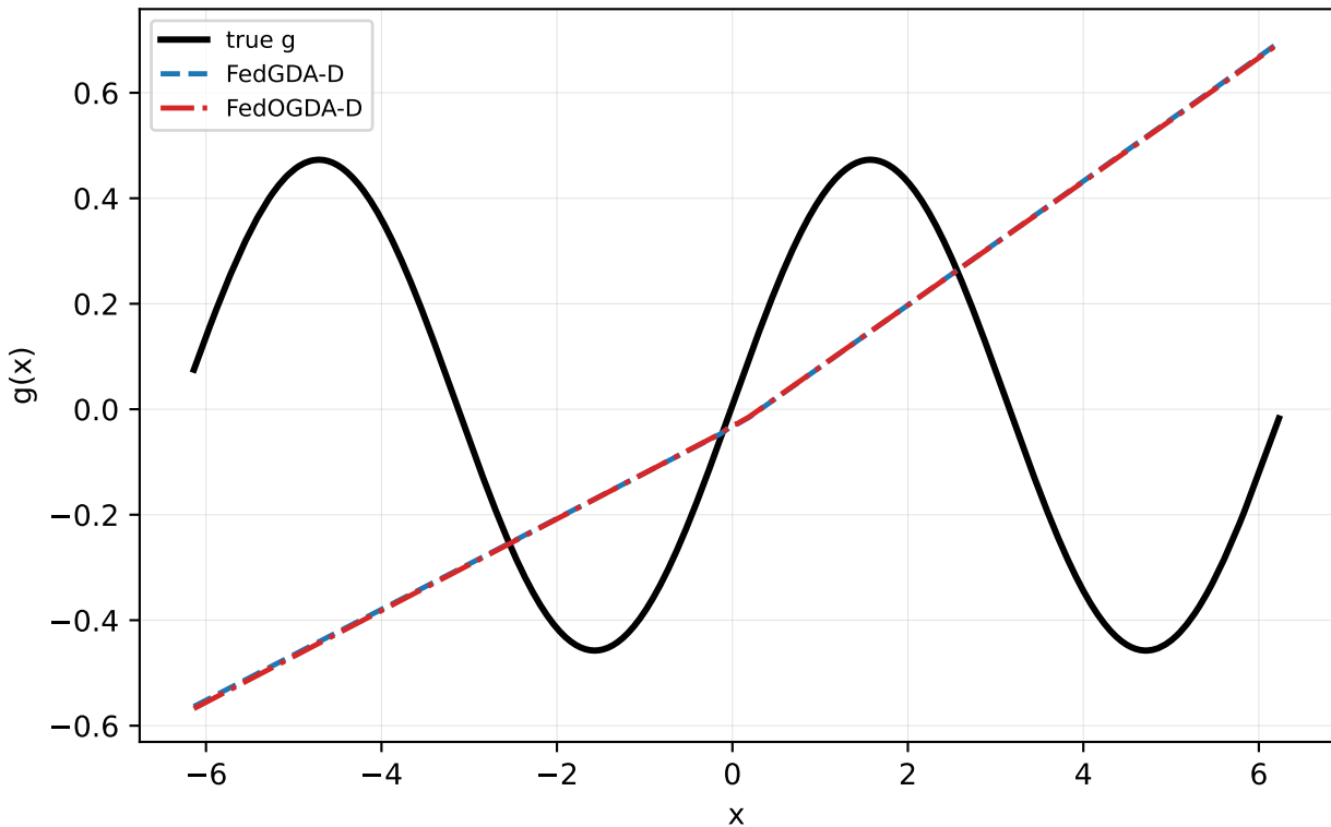
Sine \alpha=0.5 seed=0: FedGDA-D vs FedOGDA-D
