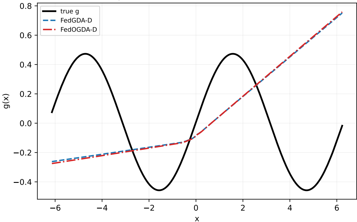
Sine \alpha=0.5 seed=2: FedGDA-D vs FedOGDA-D
