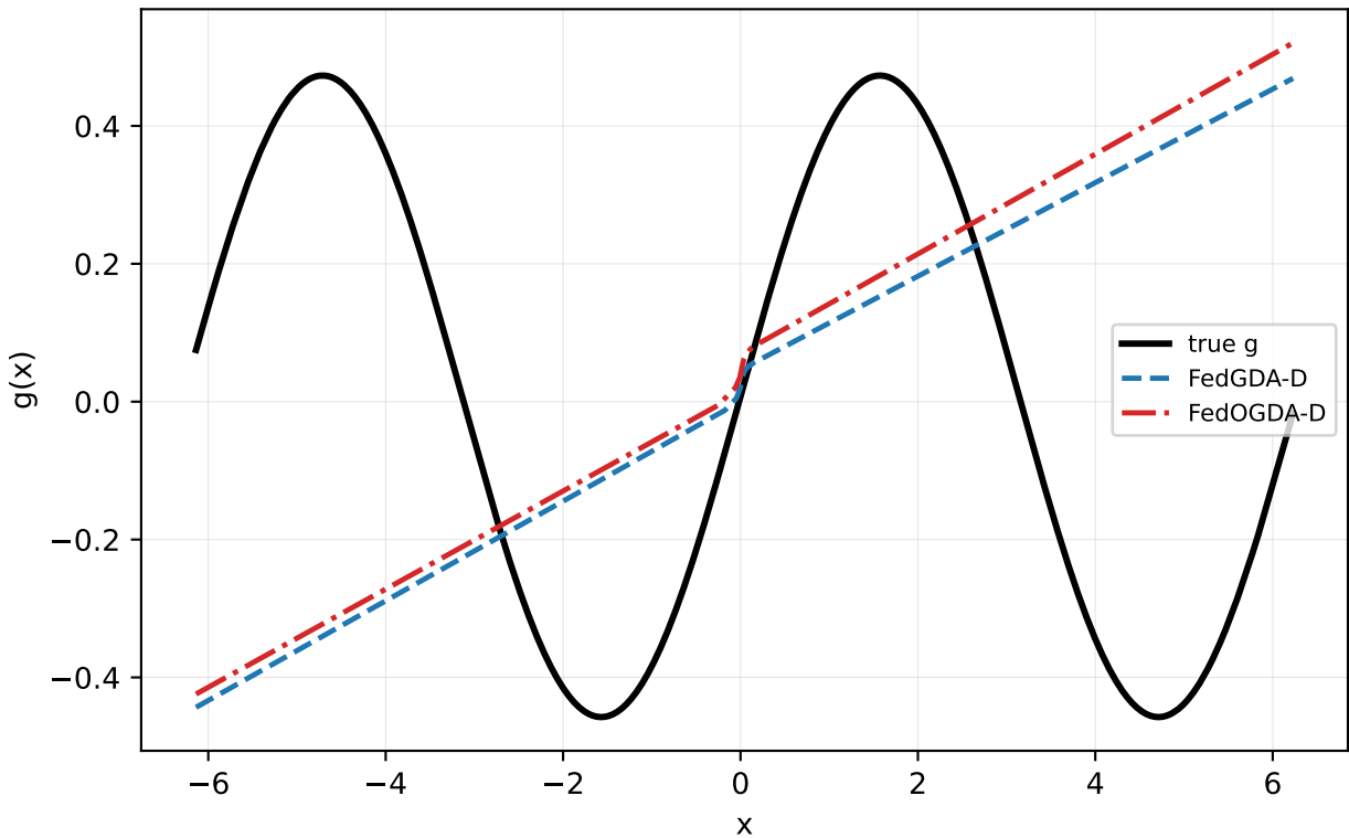
Sine \alpha=1.0 seed=1: FedGDA-D vs FedOGDA-D
