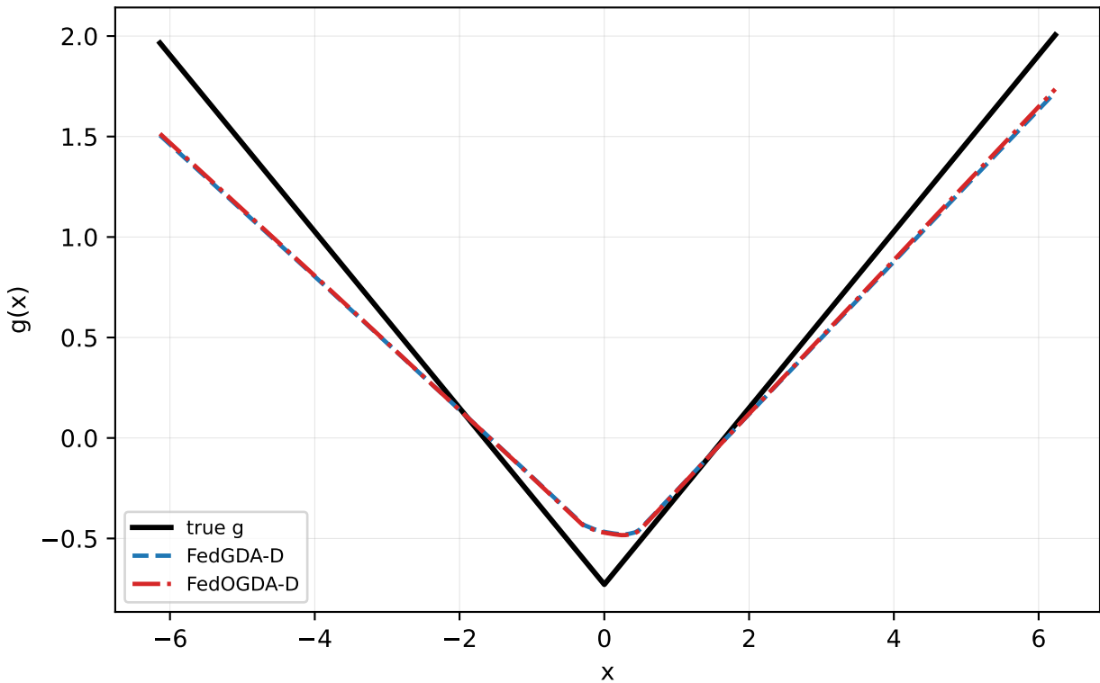
Absolute alpha=0.1: mean FedGDA-D vs FedOGDA-D
