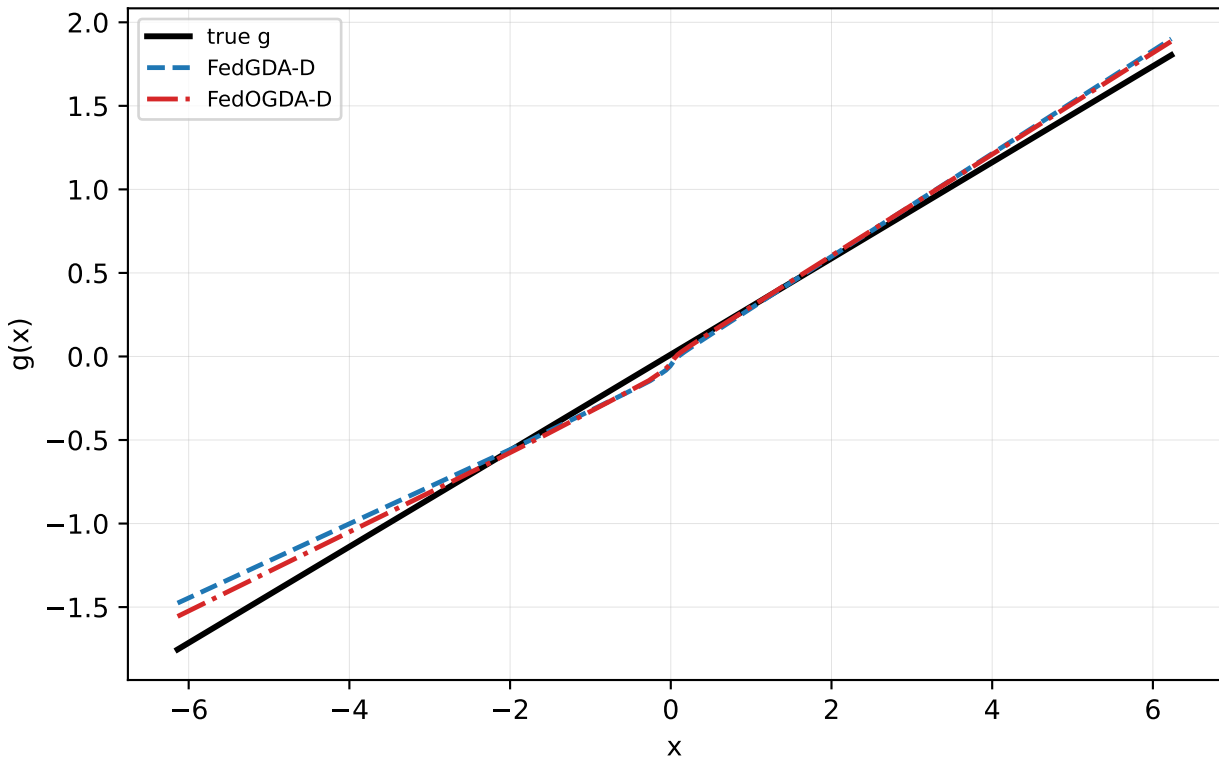
Linear \alpha=0.1 : mean FedGDA-D vs FedOGDA-D
