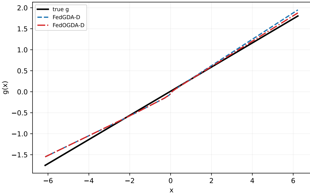
Linear \alpha=0.5 : mean FedGDA-D vs FedOGDA-D
