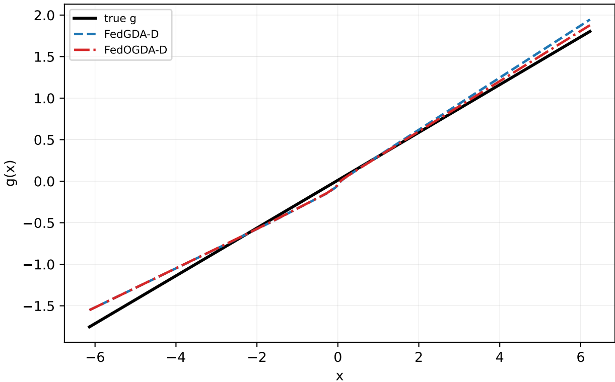
Linear \alpha=1.0 : mean FedGDA-D vs FedOGDA-D
