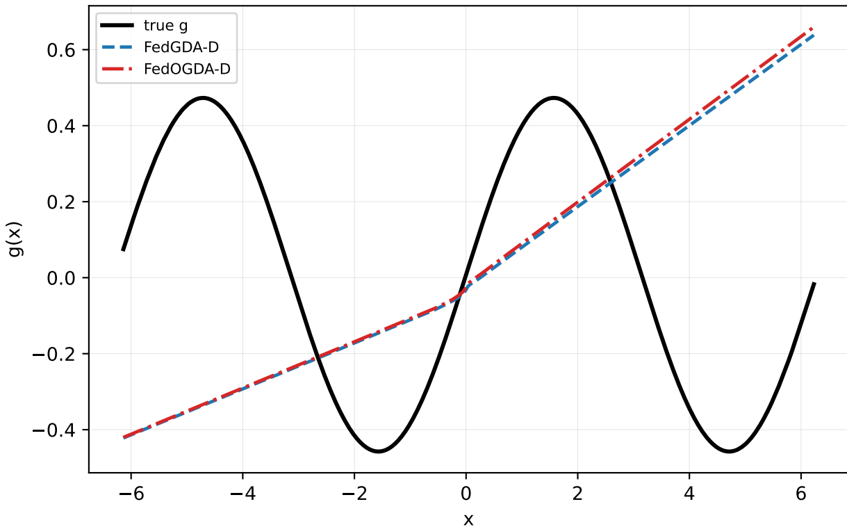
Sine \alpha=0.1 : mean FedGDA-D vs FedOGDA-D
