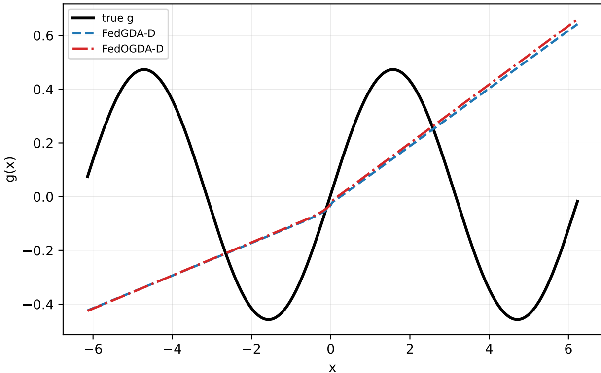
Sine \alpha=0.5 : mean FedGDA-D vs FedOGDA-D
