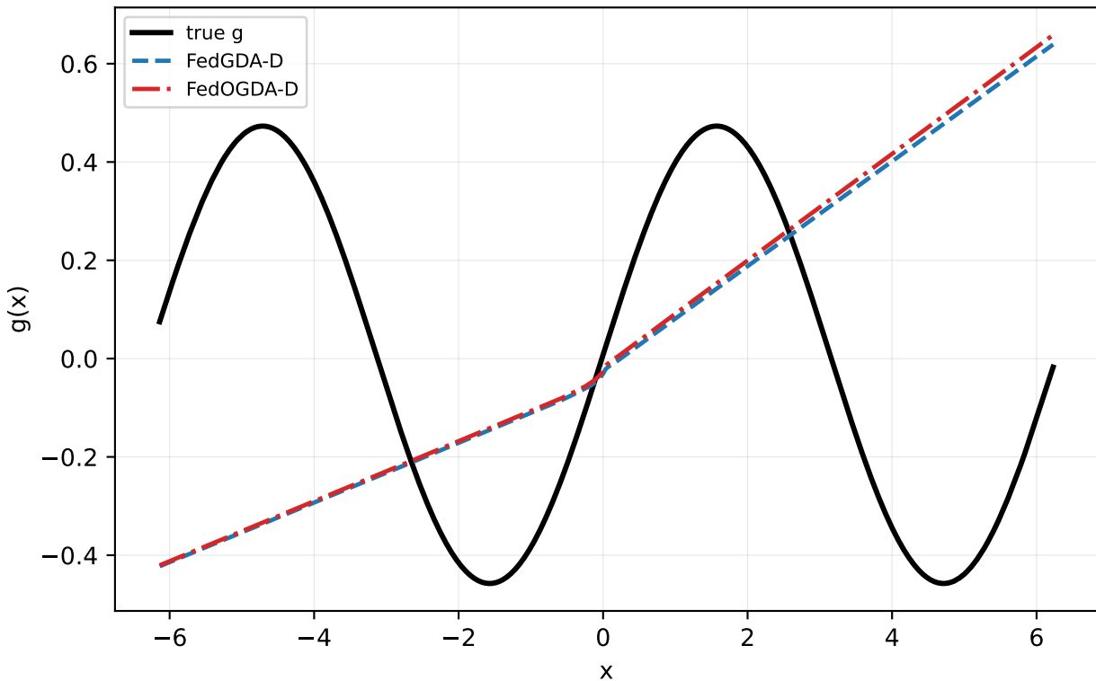
Sine alpha=1.0: mean FedGDA-D vs FedOGDA-D
