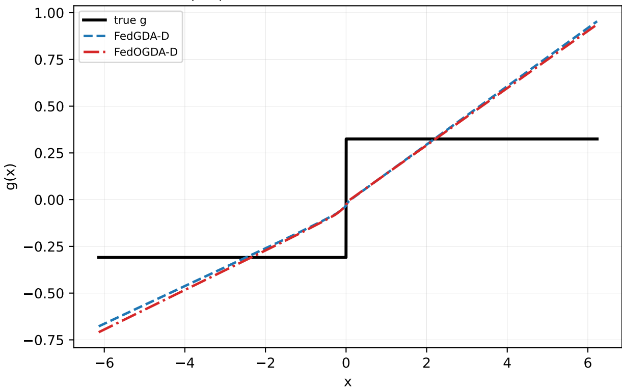
Step alpha=0.1: mean FedGDA-D vs FedOGDA-D
