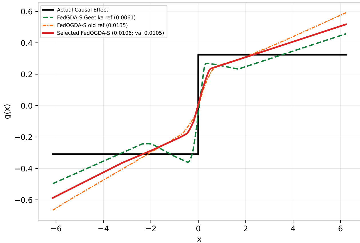
Step alpha=0.5, seed 0 selected lr=0.005, wd=0, lambda=0.1, R=7
