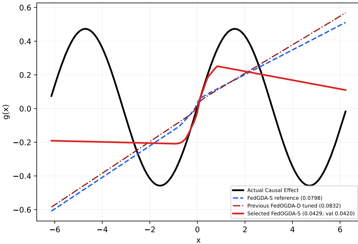
Sine alpha=1.0, seed 0 selected lr=0.005, wd=0, lambda=0.03, R=3
