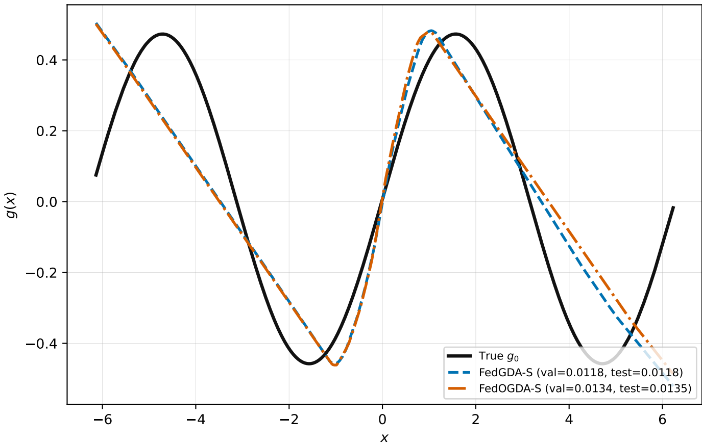
Sine, common \alpha = 0.5 : validation-selected confirmations
