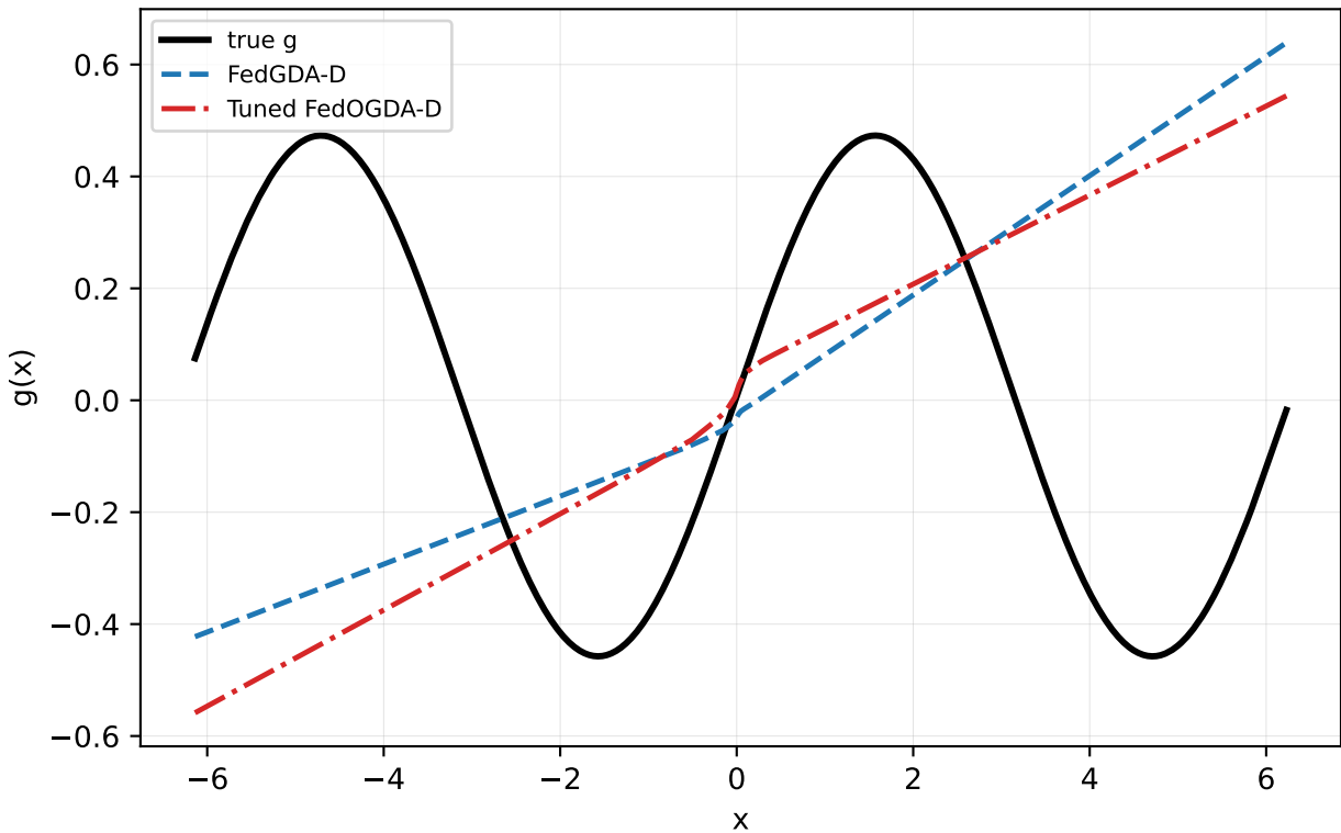
Sine tuned A2-lite: mean across seeds
