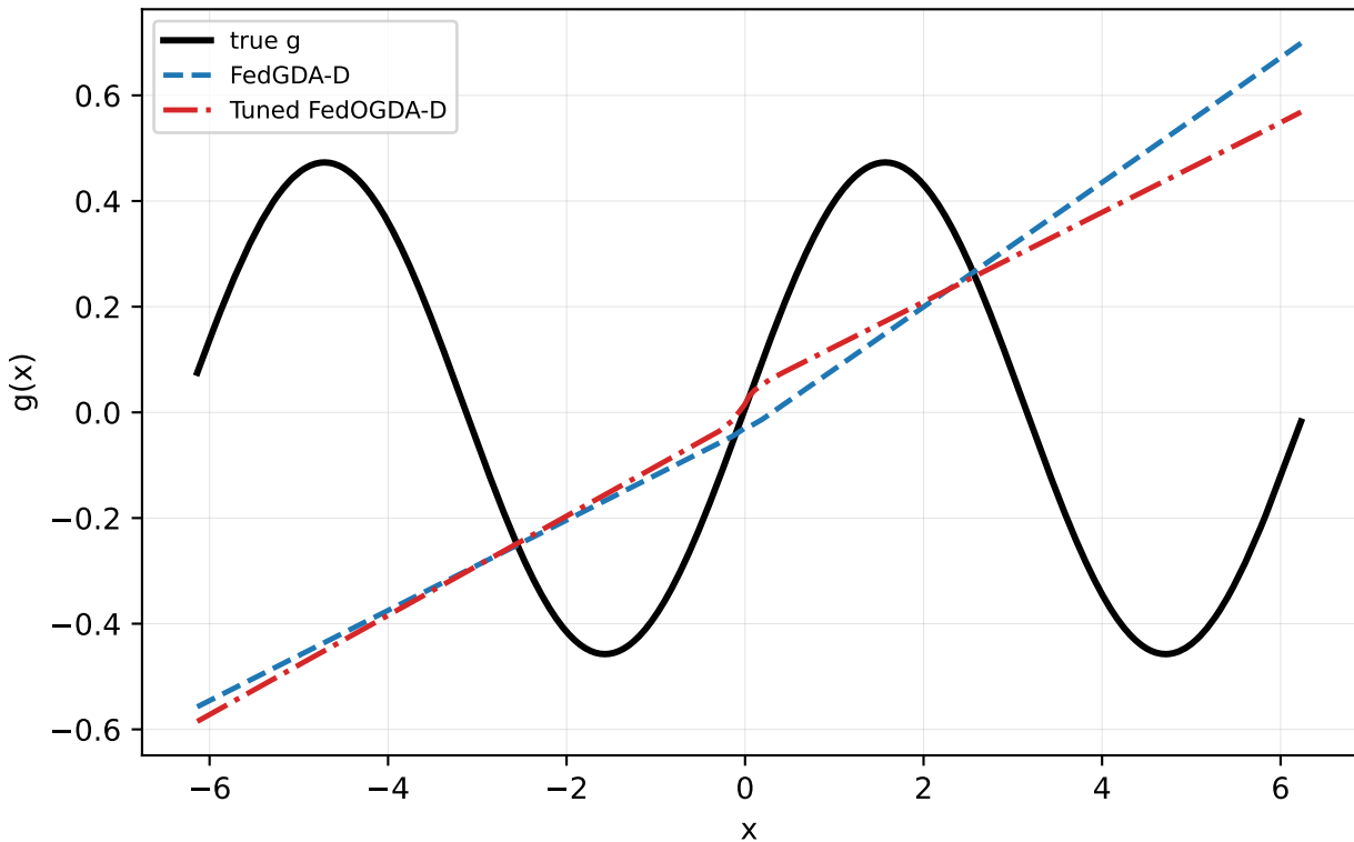
Sine tuned A2-lite seed=0: FedGDA-D vs tuned FedOGDA-D
