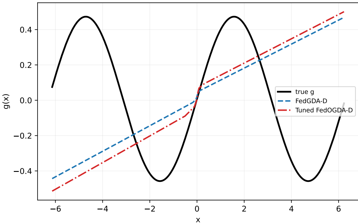
Sine tuned A2-lite seed=1: FedGDA-D vs tuned FedOGDA-D
