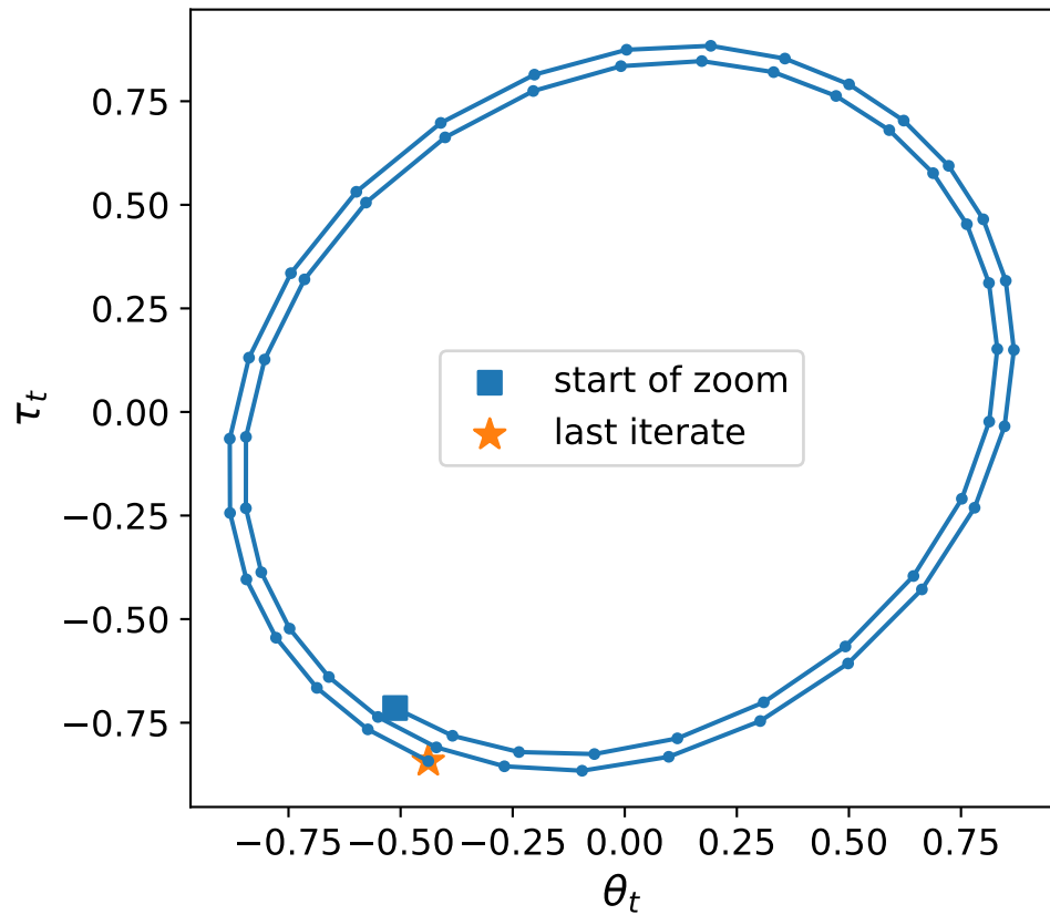
FedGDA last 60 iterates
