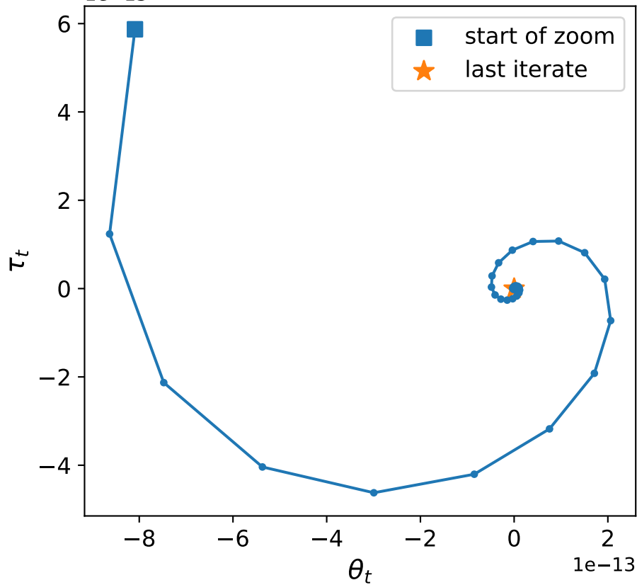
1e-13 FedOGDA last 60 iterates
