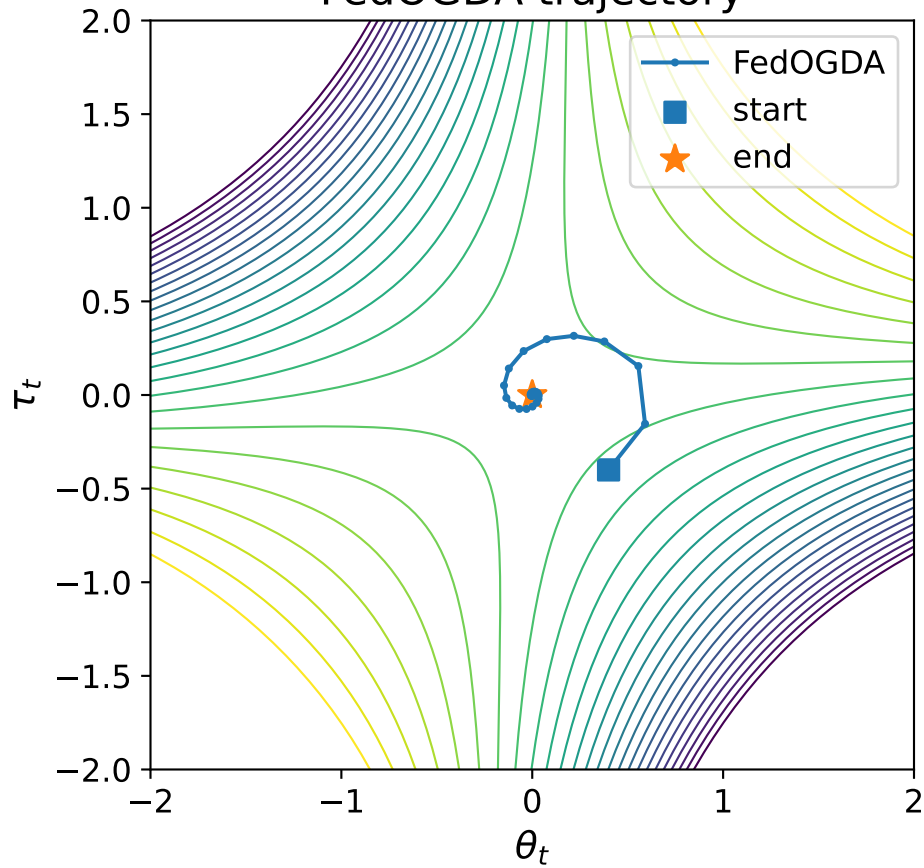
FedOGDA trajectory
