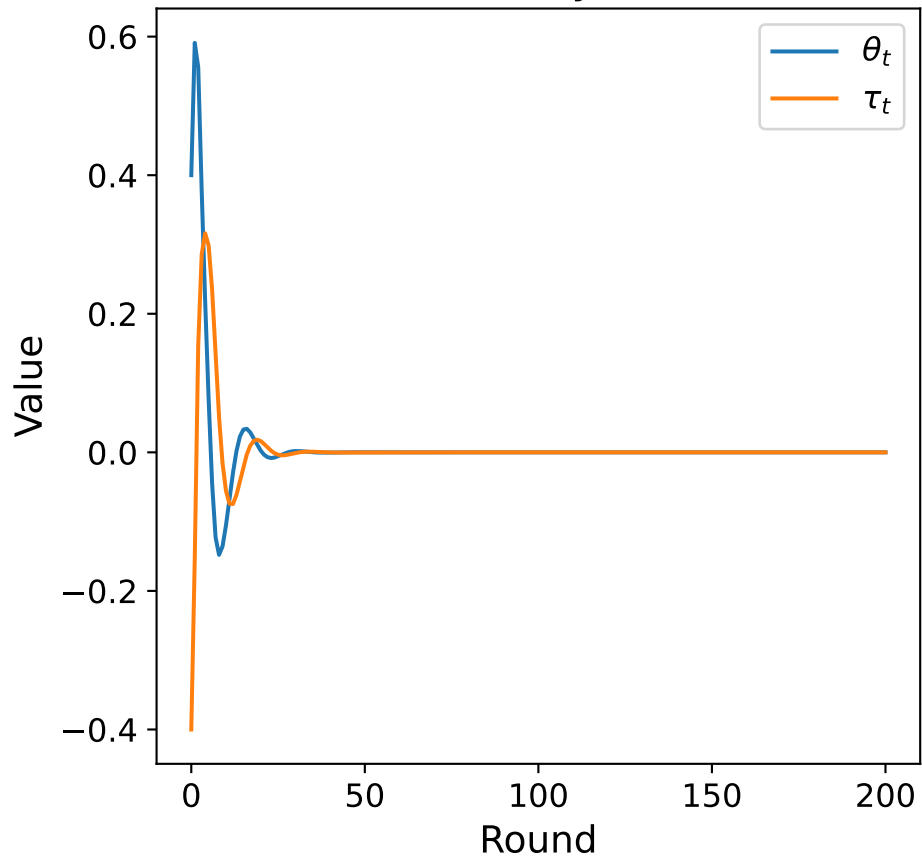
FedOGDA dynamics
