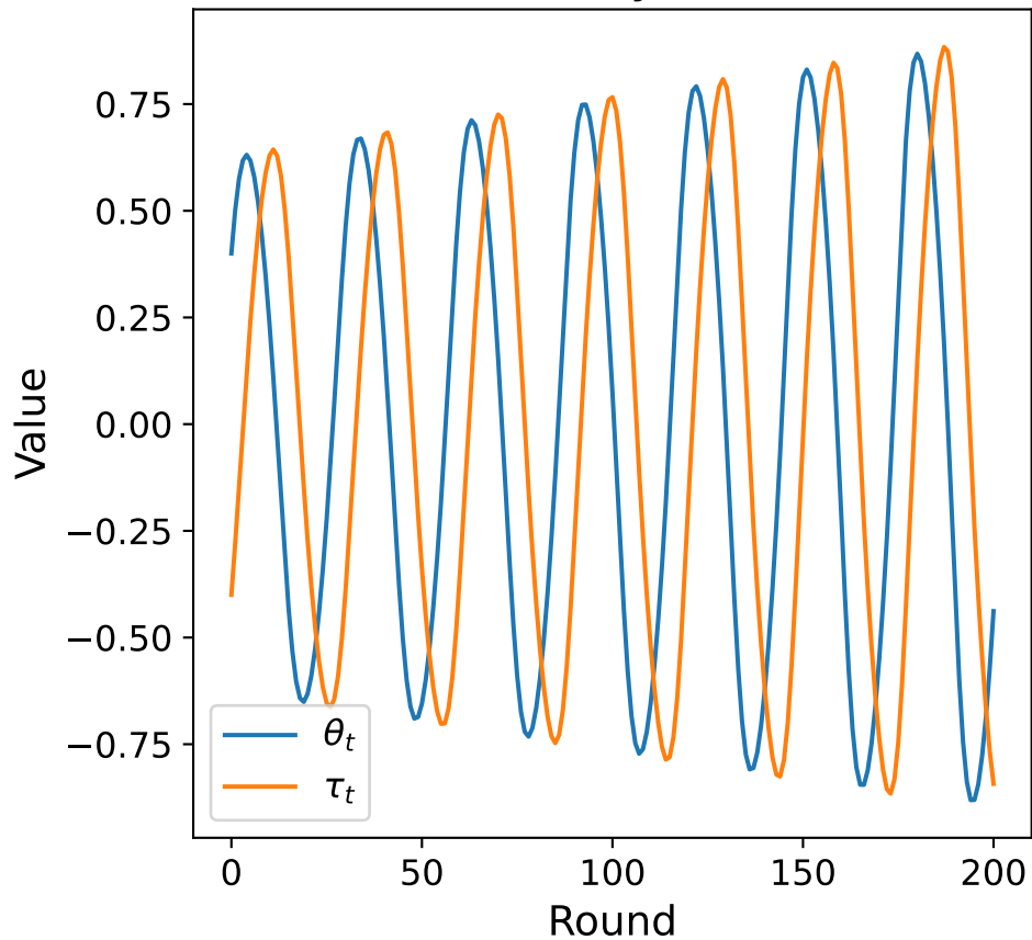
FedGDA dynamics
