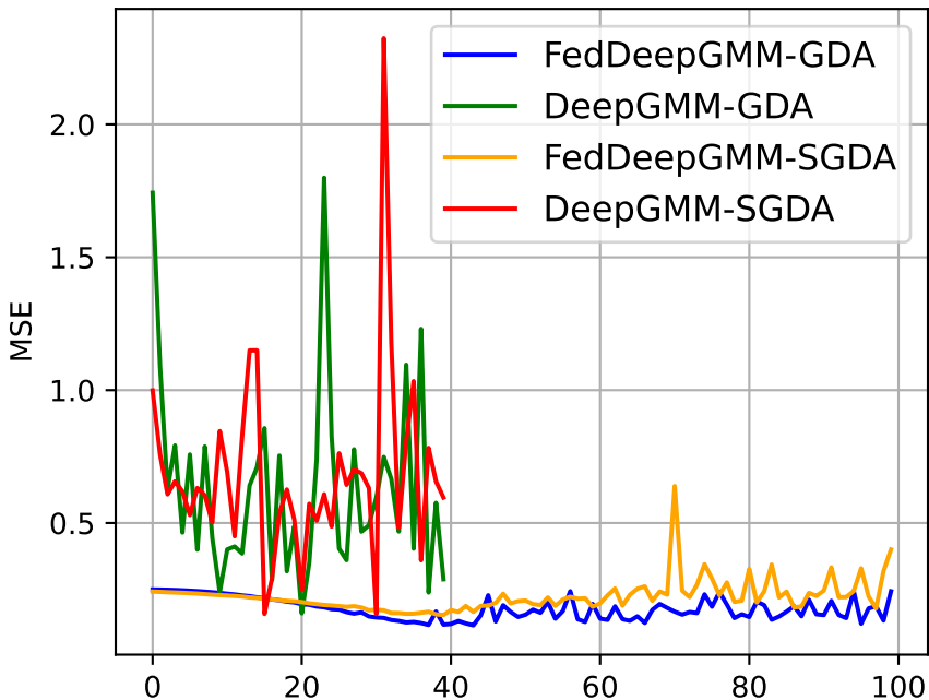
Comparison of MSE Over Rounds
