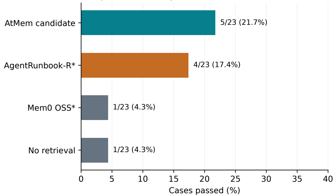
LongMemEval-V2 | 23 / 451 questions
