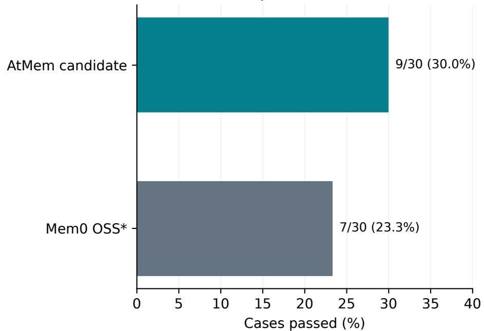
DolphinBench | 30 / 600 tasks
